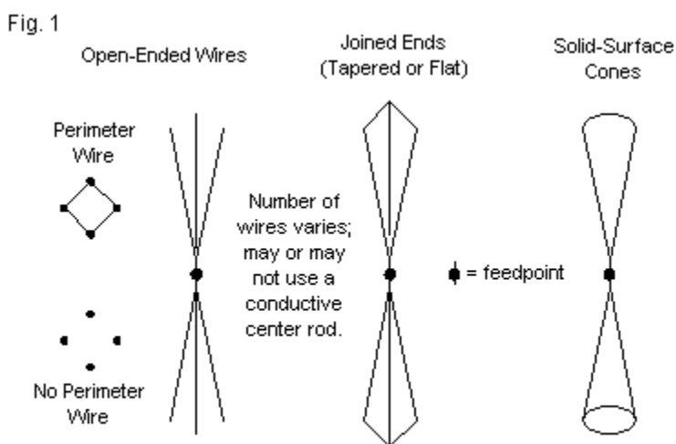
Some Biconical Configurations Used at VHF and UHF
