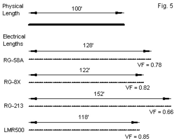
Transmission Line: Physical vs. Electrical Lengths
