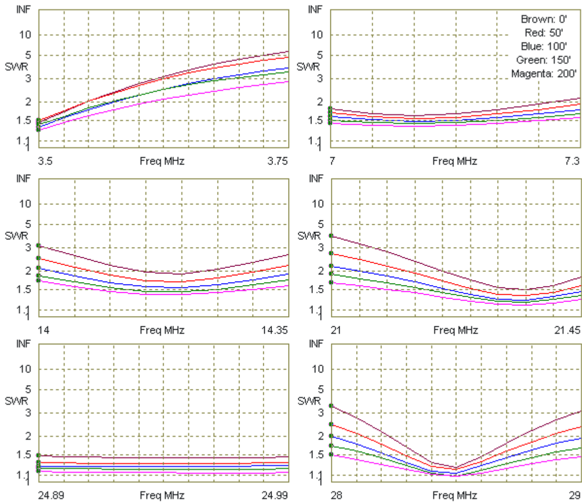
In-Band 50-Ohm SWR Sweeps: OCF Antenna and RG-58A Cable 50' above Average Ground
