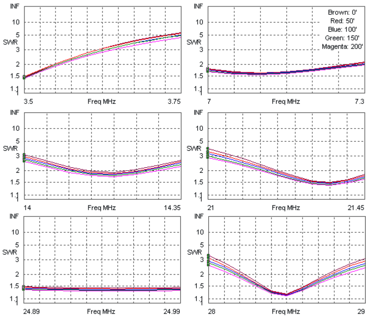
In-Band 50-Ohm SWR Sweeps: OCF Antenna and LMR500 Cable 50' above Average Ground
