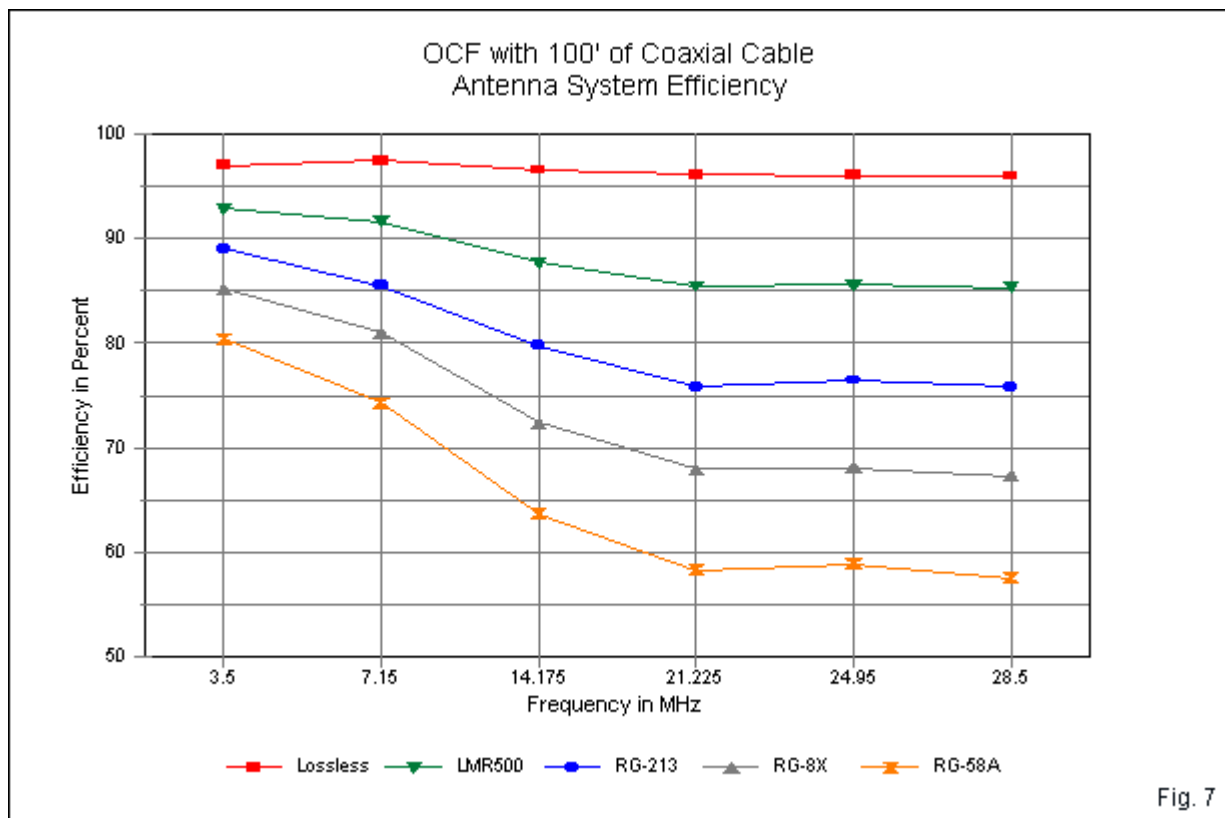
Fig. 7 graphs the efficiency levels for each cable and includes the values for the no cable situation, which is equivalent to using a hypothetical 100' cable with no losses at all. Besides variations in wire losses due to varying skin effects at the different frequencies, we see other fluctuations in the graphed lines. Cable losses are a combination of two factors. One is the
