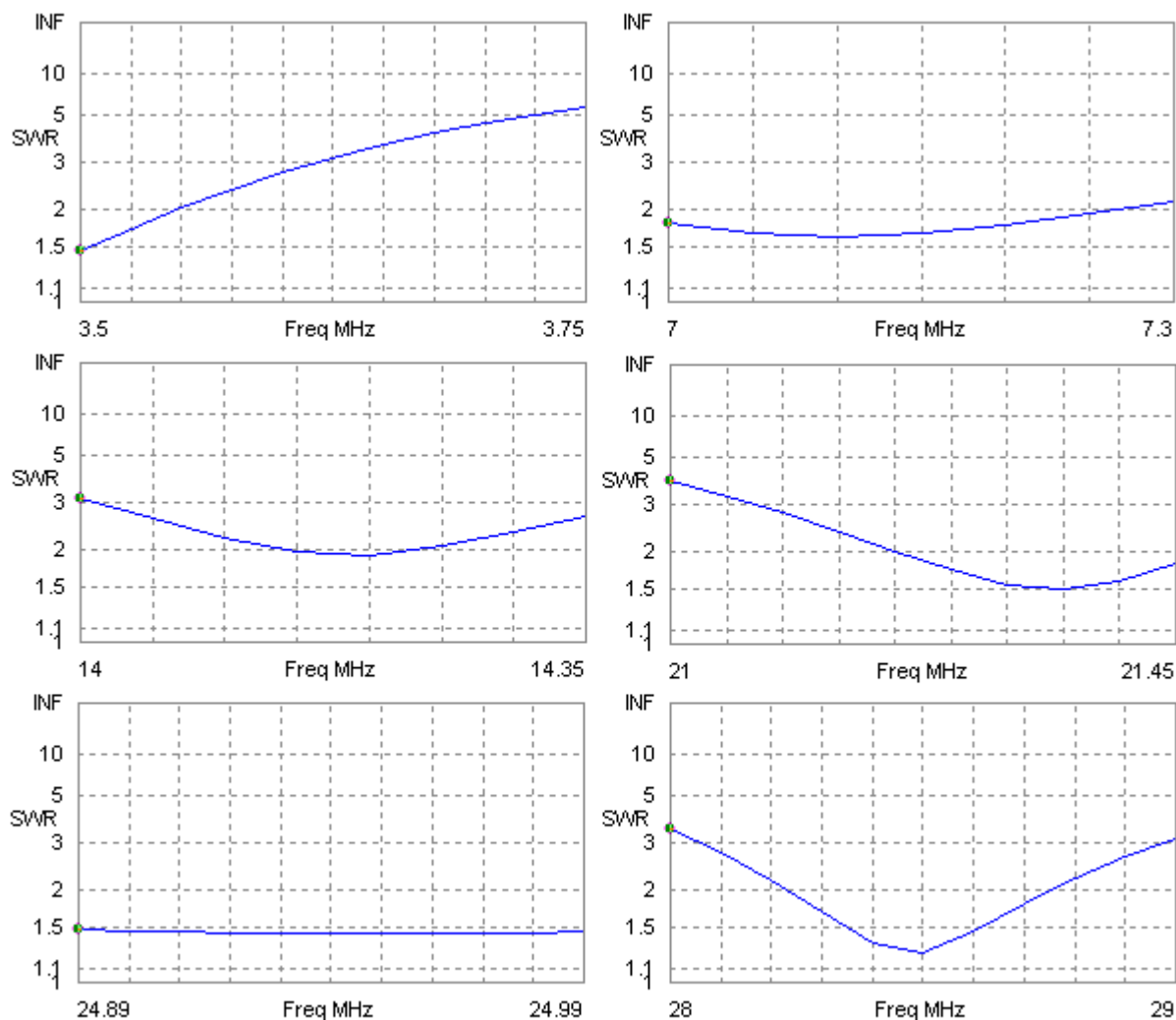
In-Band 50-Ohm SWR Sweeps: OCF Antenna 50' above Average Ground
