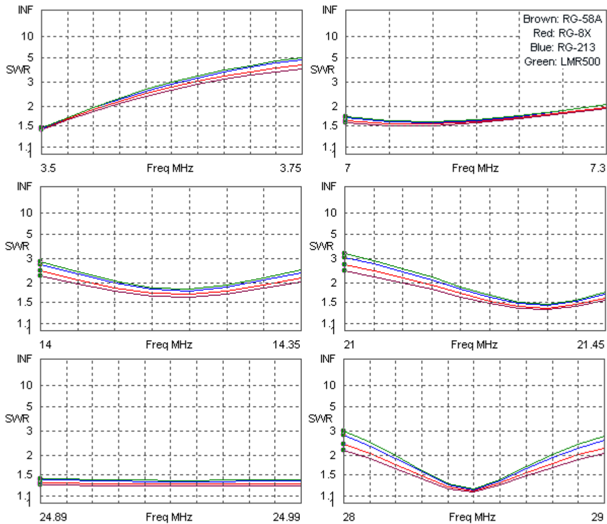
In-Band 50-Ohm SWR Sweeps: OCF Antenna and Cables 50' above Average Ground Fig. 6
