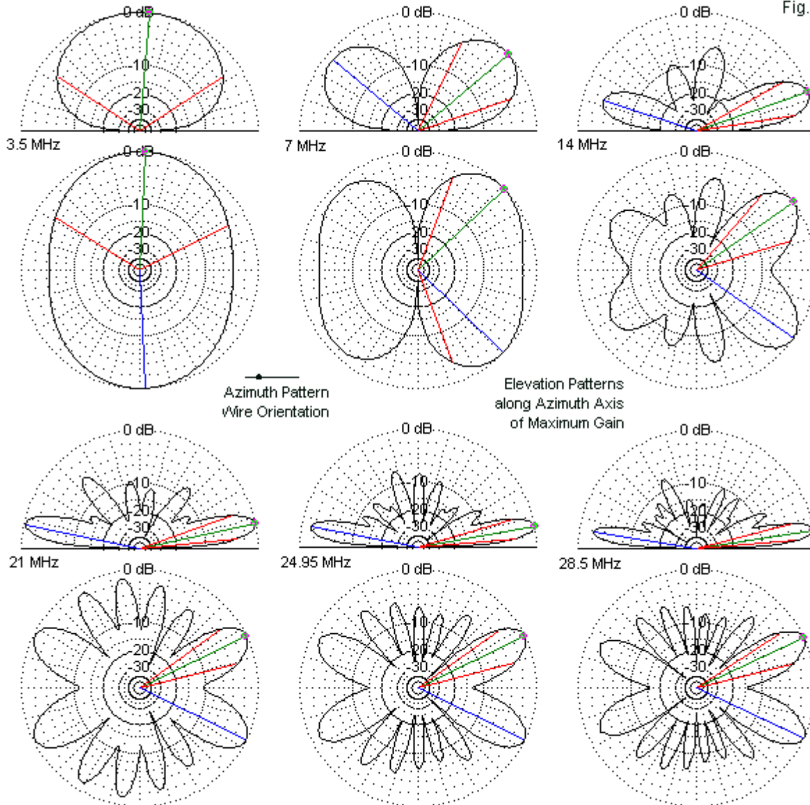
Elevation and Azimuth Patterns: Isolated OCF at 50' above Average Ground
