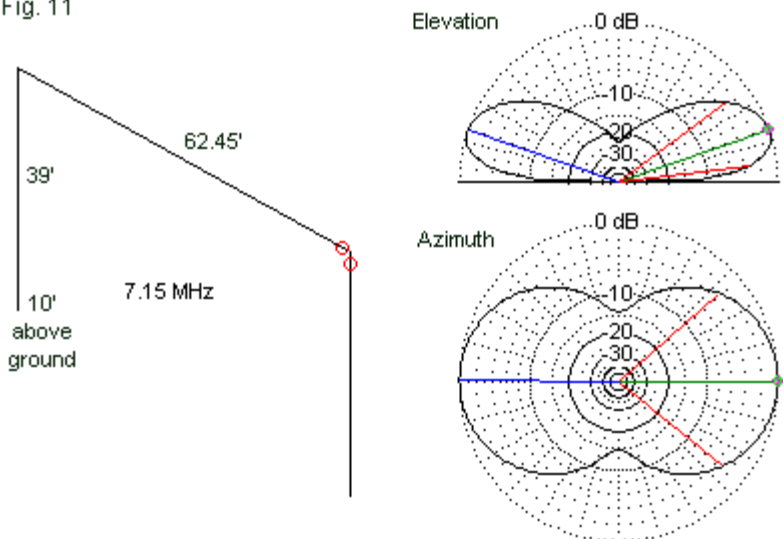
Outlines and Radiation Patterns of a Half-Square Array
