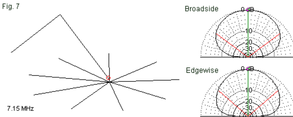
Outline and Radiation Patterns of a Half-Loop with One End Ungrounded
