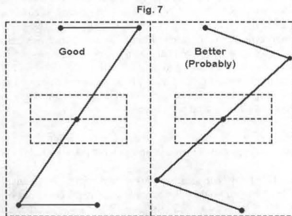
Two Configurations of a 135' Doublet: Zig-Zagged
