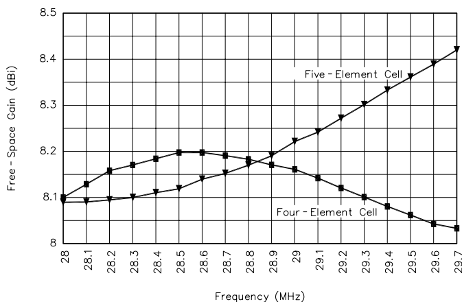
Fig 3—Log-cell Yagis with four-element and five-element cells: free-space gain.
