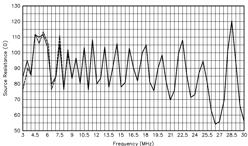
Fig 15—Source resistance of the 26-element, 164-foot LPDA model without (solid) and with (dashed) a shorted stub at 0.5 MHz intervals. See text for stub dimensions.
